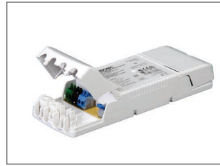
/TOP Tridonic Excite Driver - 100K hours I-Select, Loop in - loop out
